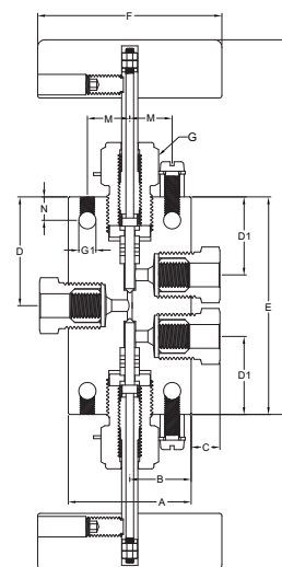
3-way/2 stem manifold
